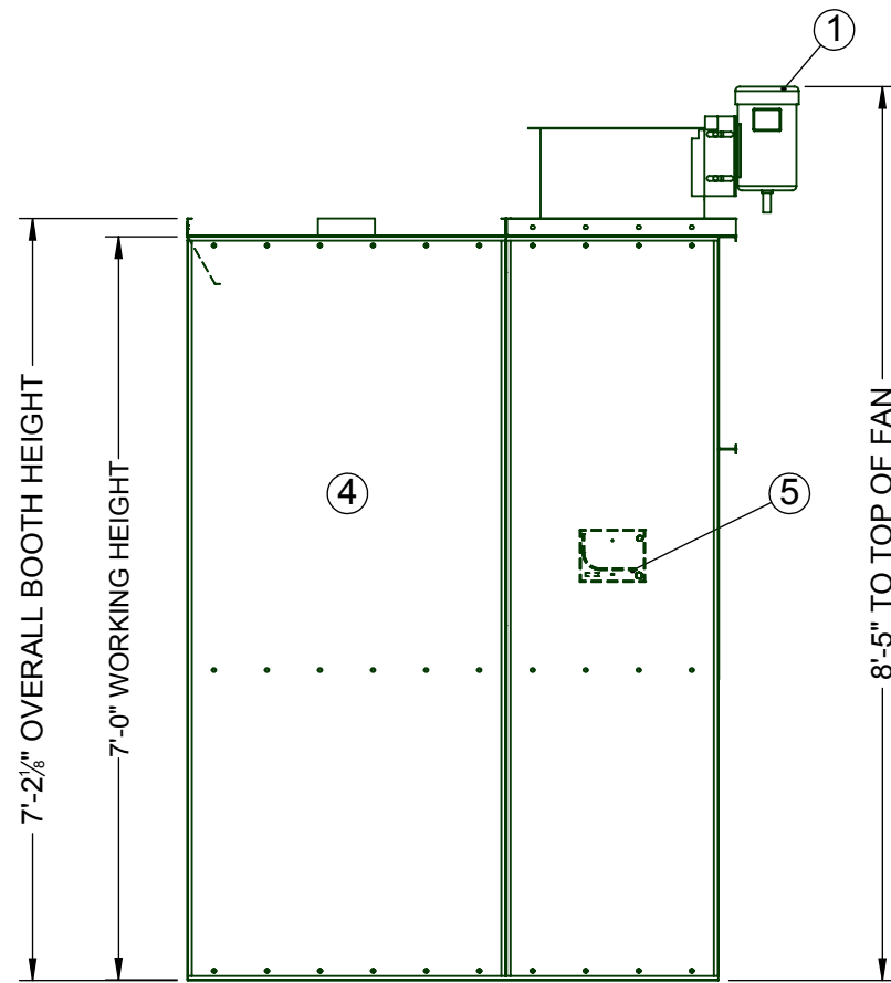
SIDE VIEW
